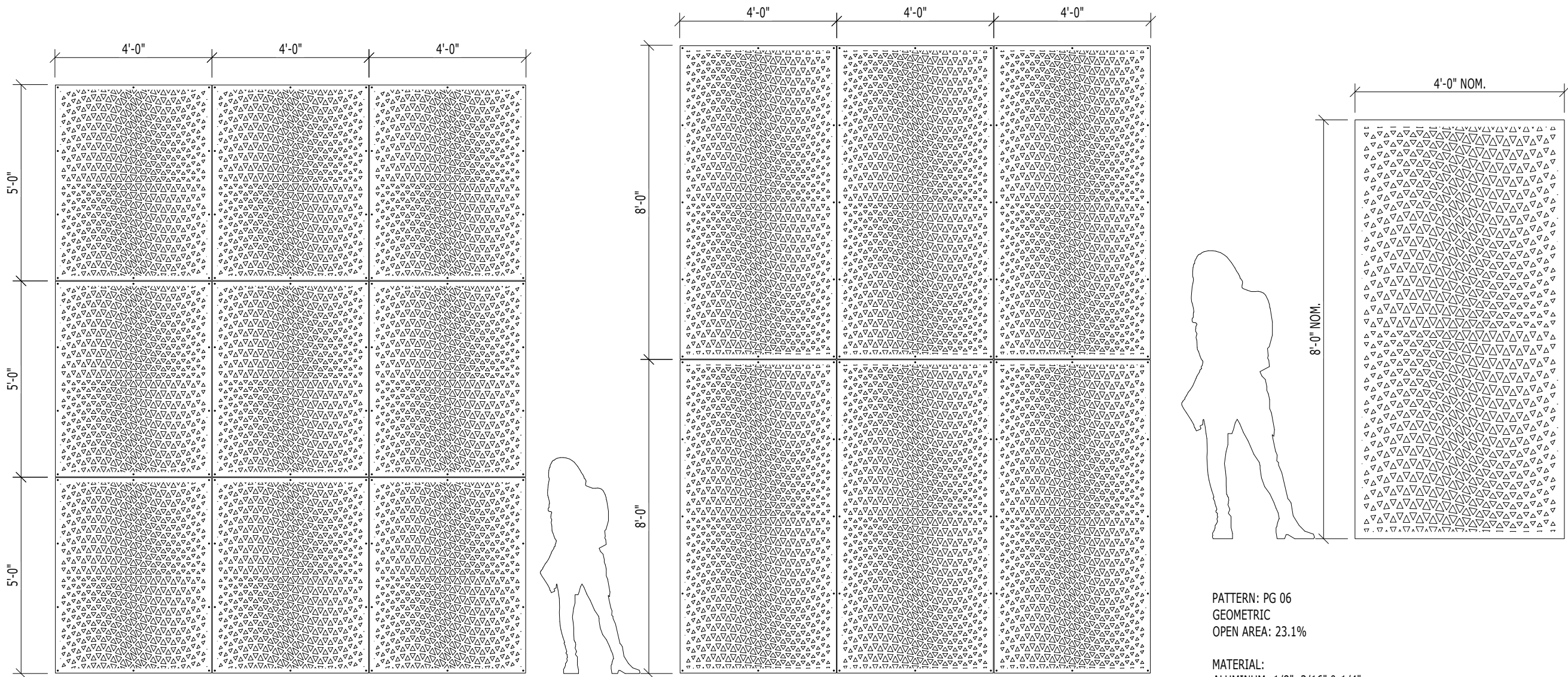
WALL SYSTEM WITH 4'-0" x 5'-0" STANDARD PANELS
