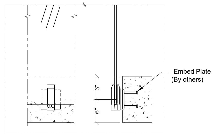
Welded @ Embed Plate - $$ Detail# ZA-F02
