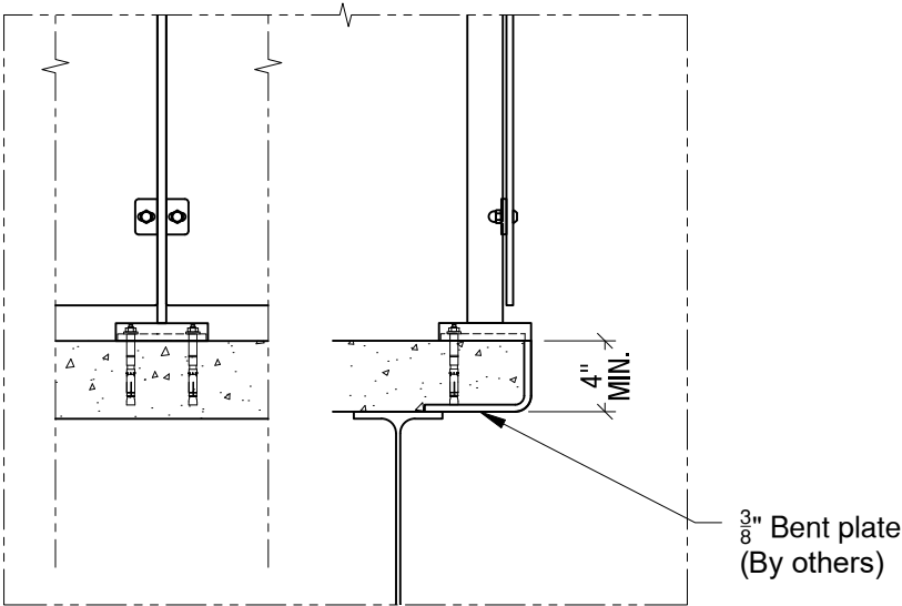
Welded @ Steel Angle Anchored @ Concrete - $$ Detail# ST-T06
