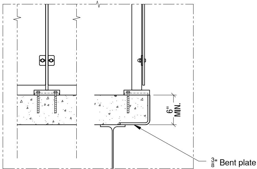
Welded @ Steel Angle Anchored @ Concrete - $$ Detail# ST-T07
