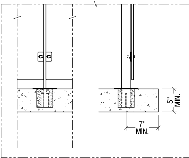
Cored into Concrete - $$ Detail# ST-T02
