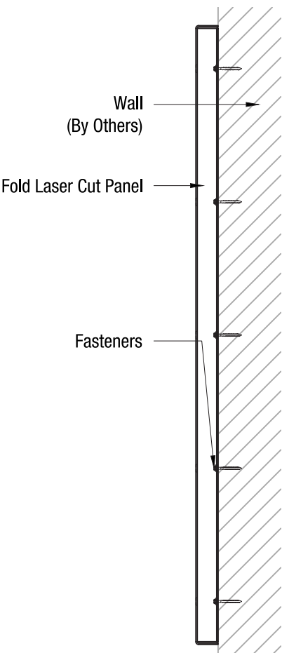
FD2-3 MOUNT TO WALL
