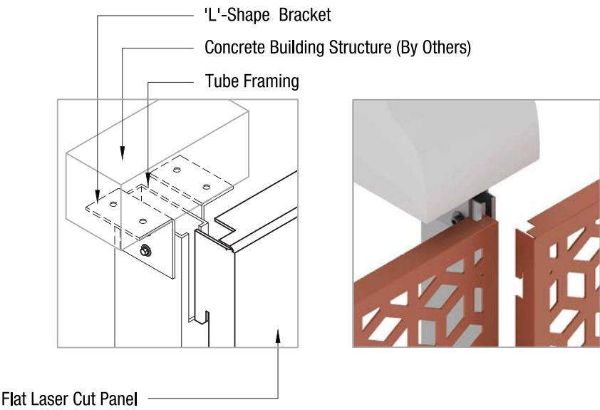
FD1-6 BETWEEN CONCRETE SLAB (INSET)
