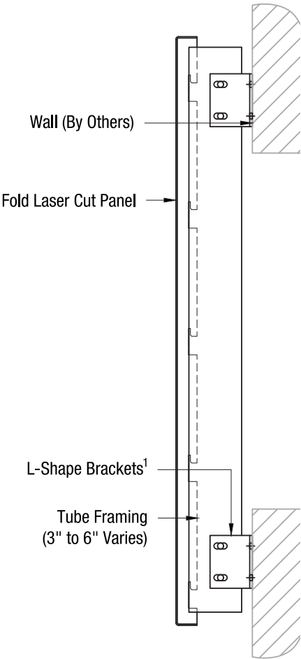
FD1-4 BETWEEN FLOOR LEVELS
