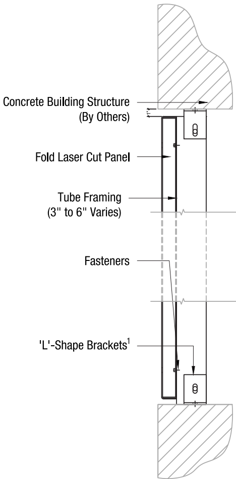
FD2-6 BETWEEN CONCRETE SLABS (INSET)
