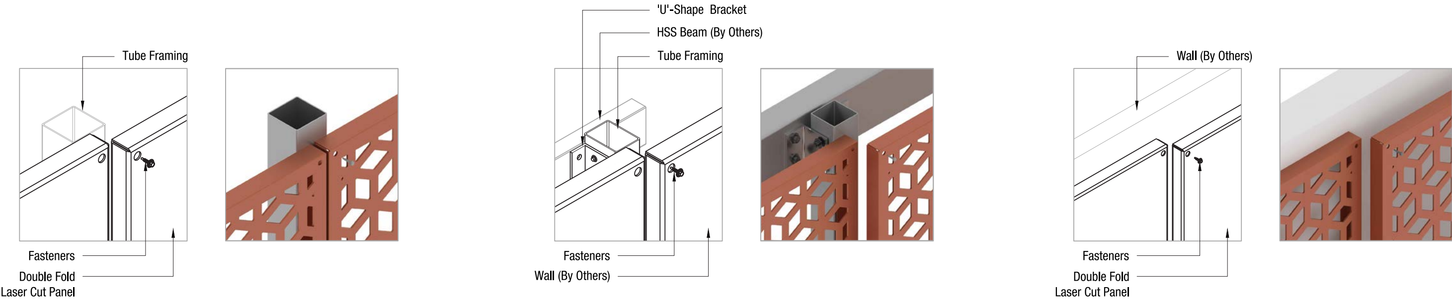
FD2-1 TO STEEL COLUMN
