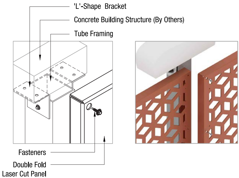
FD2-6 BETWEEN CONCRETE SLABS (INSET)
