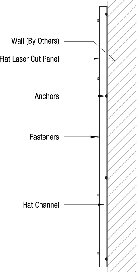
FLT-2 TO BUILDING STRUCTURE
