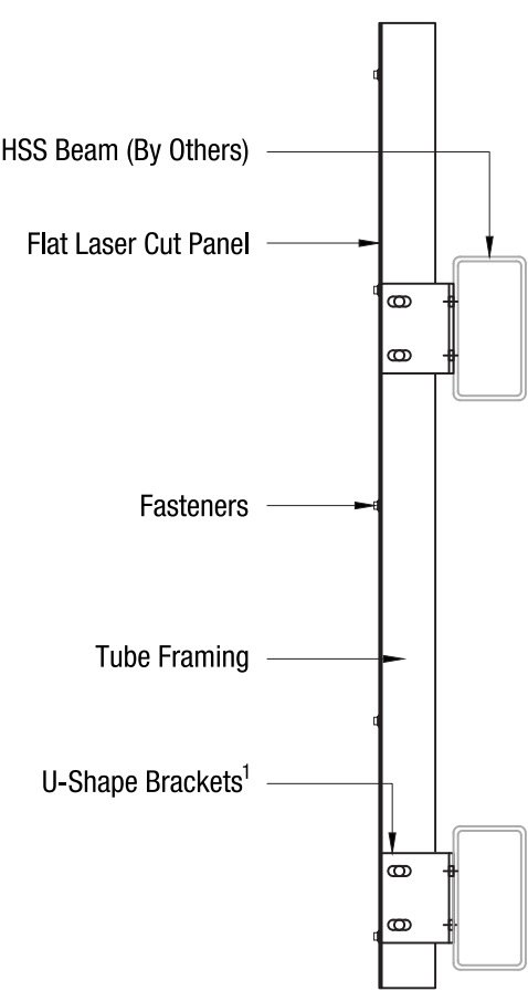
FLT-1 TO STEEL BEAM
