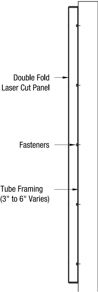
FD2-1 TO STEEL COLUMN
