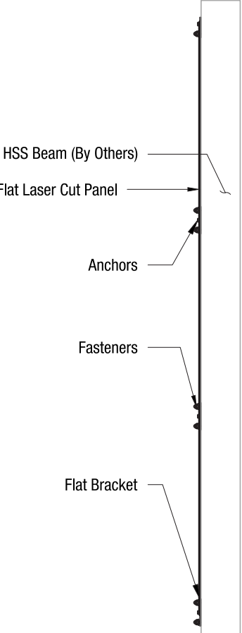
FLT-3 TO FRAMING
