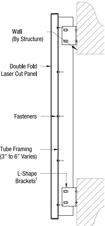
FD2-4 BETWEEN FLOOR LEVELS
