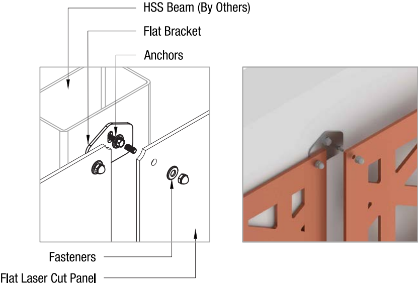
FLT-3 TO FRAMING
