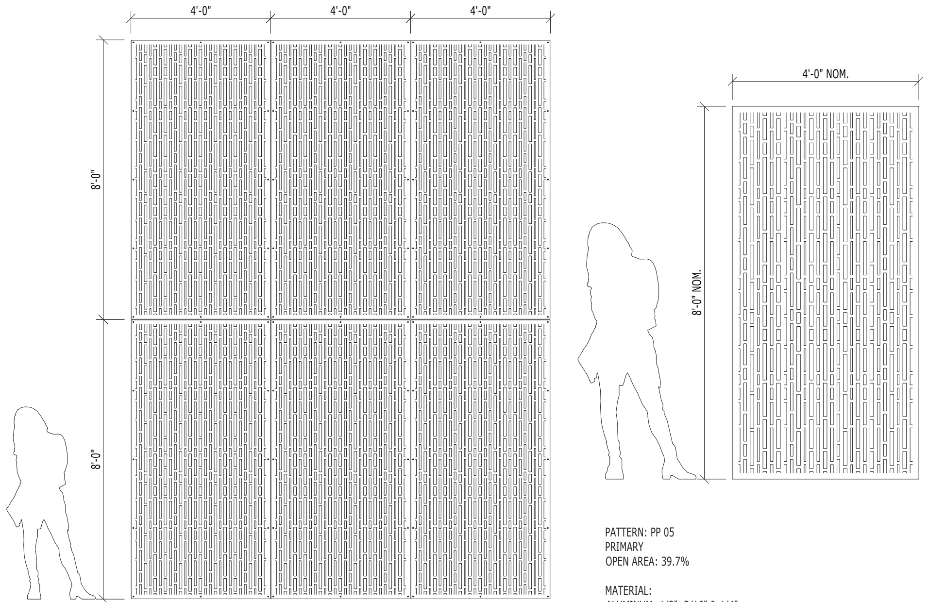
WALL SYSTEM WITH 4'-0" x 8'-0" STANDARD PANELS
