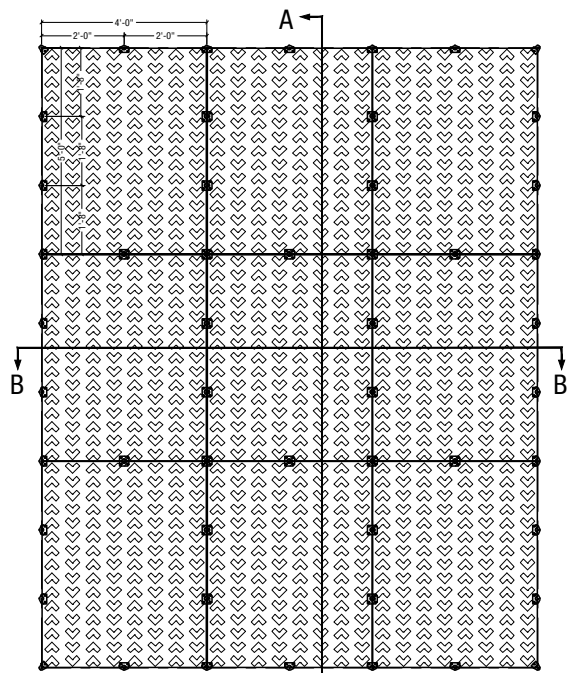
Panel Array Layout Elevation View
