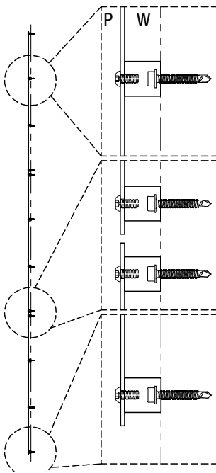
Fastener Section Detail (A-A) Vertical Alignment
