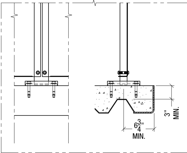
Anchored to Concrete Slab on Deck - $$ Detail# F0-T05
