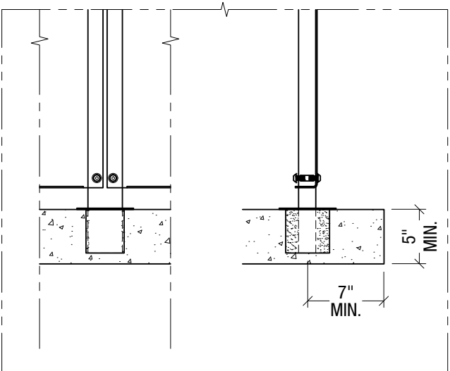
Cored into Concrete - $$ Detail# F0-T02
