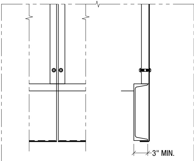
Welded @ Steel Channel - $ Detail# F0-T03
