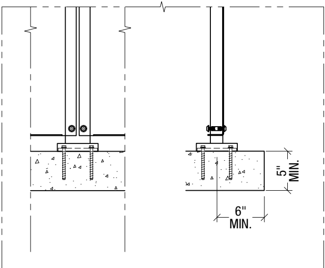
Anchored to Concrete 1 - $ 2 Detail# F0-T01
