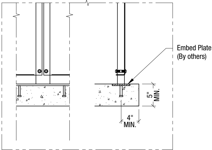
Welded @ Embed Plate - $ Detail# F0-T04
