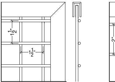
WM-38ST (Welded Steel)
