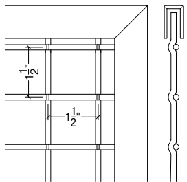
WM-38ST (Welded Steel)
