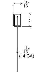
SECTION VIEW
