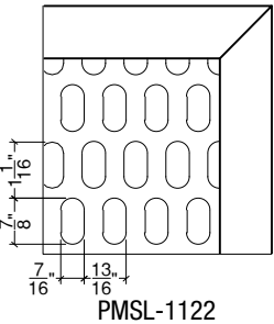
SECTION VIEW
