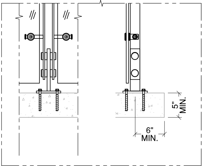
Anchored to Concrete 1 - $ 2 Detail# BL-T01 3
