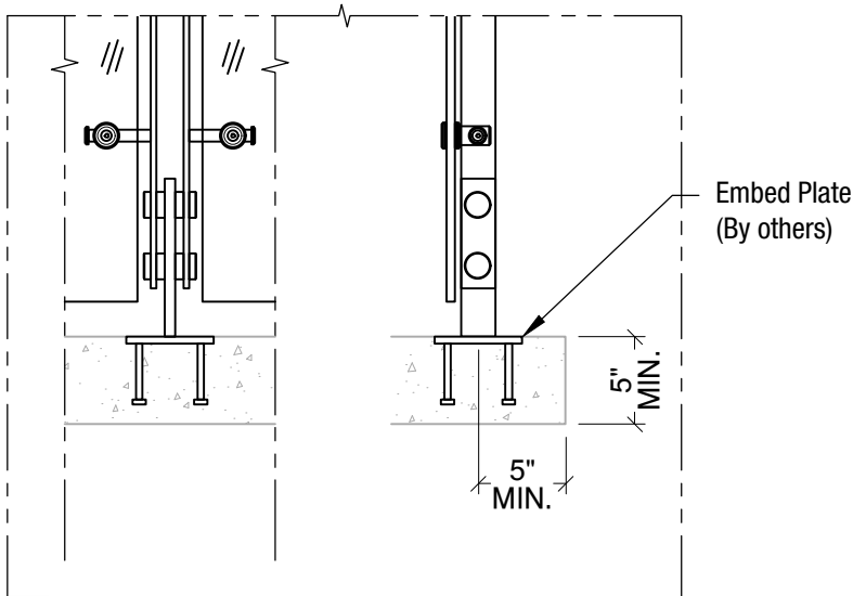
Welded @ Embed Plate - $ Detail# BL-T04
