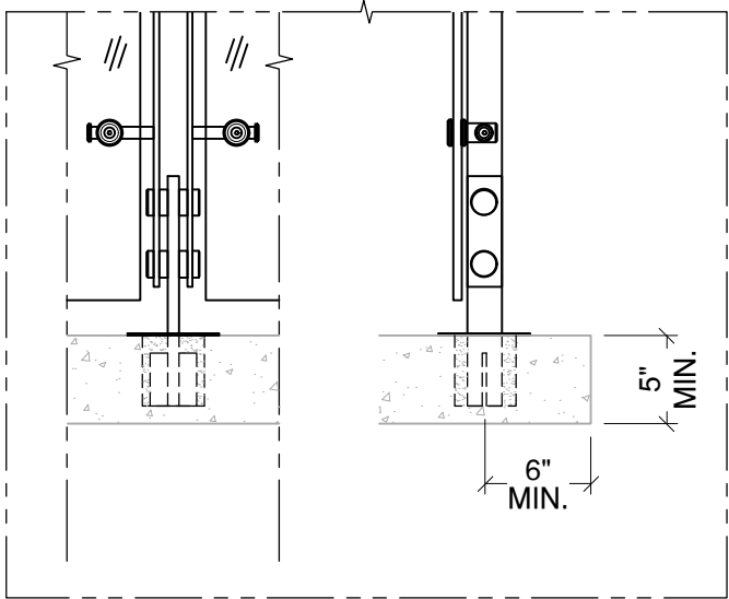
Cored into Concrete - $$ Detail# BL-T02
