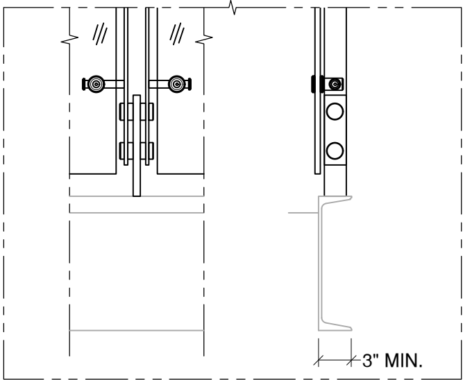
Welded @ Steel Channel - $ Detail# BL-T03
