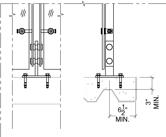
Anchored to Concrete Slab on Deck - $$ Detail# BL-T05
