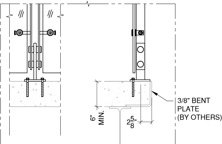
Anchored to Concrete Welded to Steel Plate - $ Detail# BL-T06
