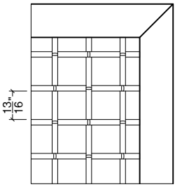
WM-20SS (Woven SS)
