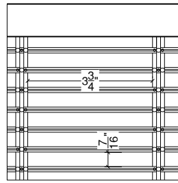
WM-11SS (Woven SS)
