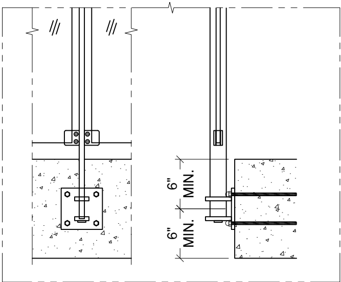
Anchored to Concrete 1 - $$$ Detail# BE-F01 2
