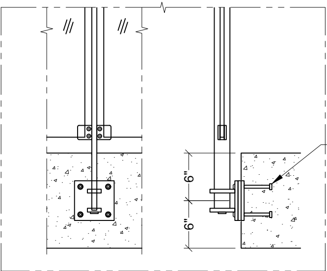
Welded @ Embed Plate - $$ Detail# BE-F02
