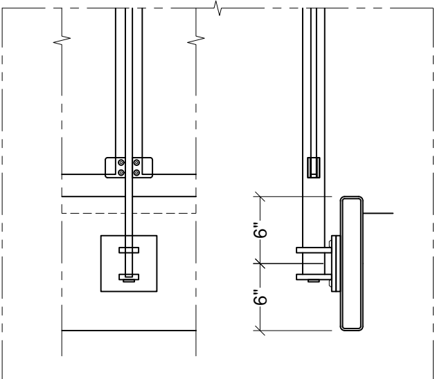
Welded @ Steel Tube - $$ Detail# BE-F04
