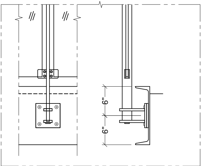
Welded @ Steel Channel - $$ Detail# BE-F03
