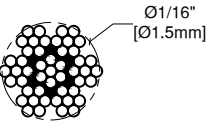
7x7 CONSTRUCTION CABLE
