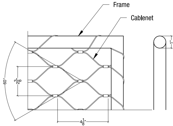
DIMENSIONS ARE NOMINAL
