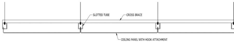
SECTION - HOOK SYSTEM, SLIDE AND LOCK
