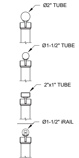
TOP RAIL OPTIONS
