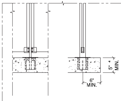
Cored into Concrete - $$
